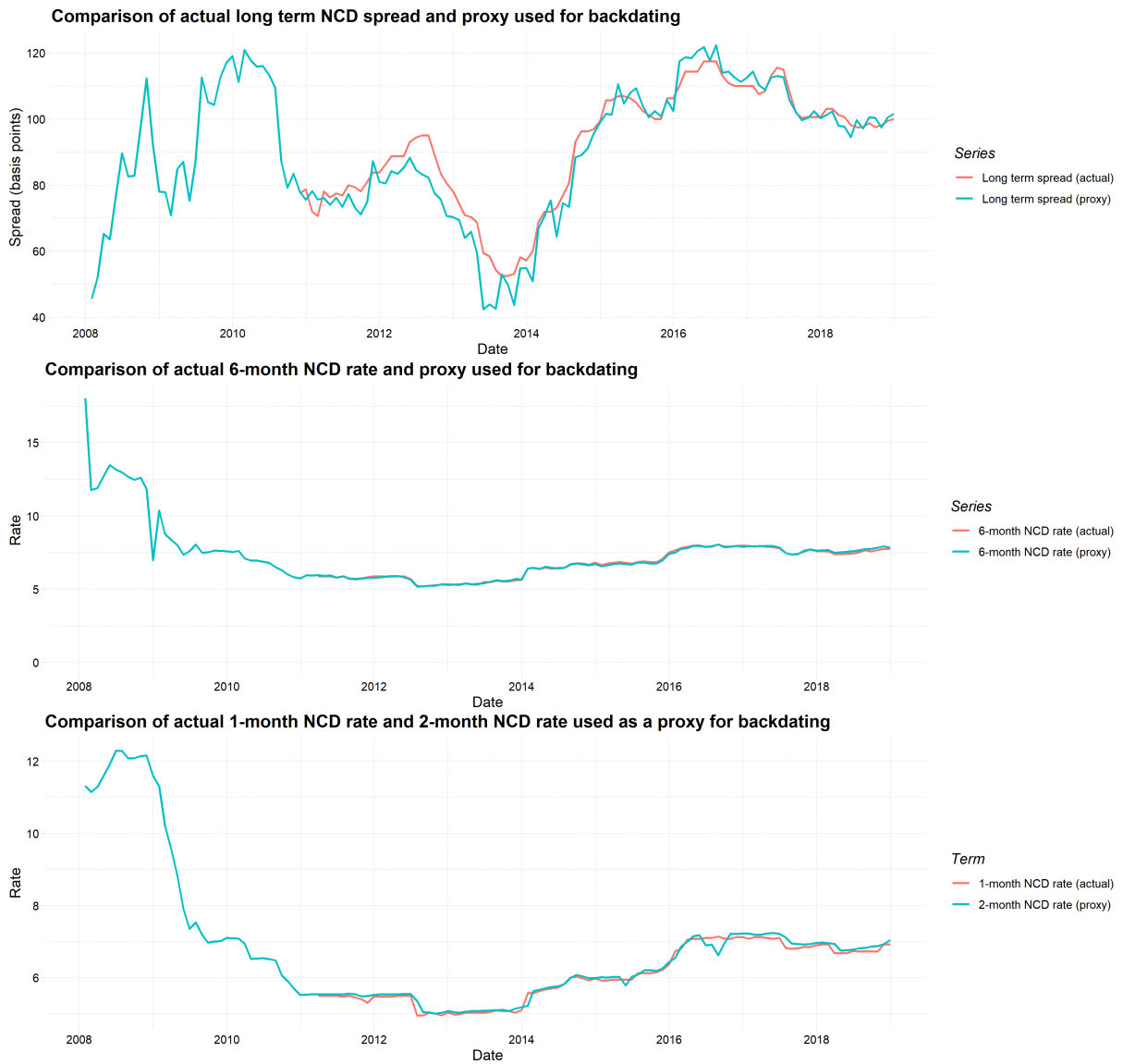
Figure 21: Backdating NCD
